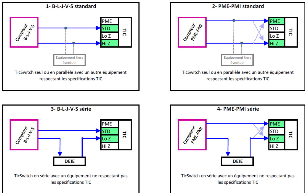
Figure 4: schéma de raccordement
