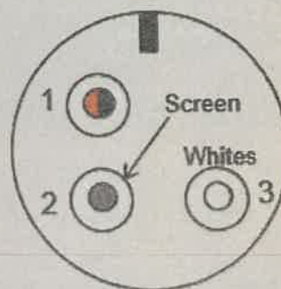
Figure 7 Modbus Connector Cable Part - Binder 99-9210-00-04 (Front View)
