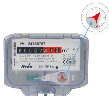
Pre-equipped register with the Cyble Target
