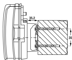
Fixation murale
